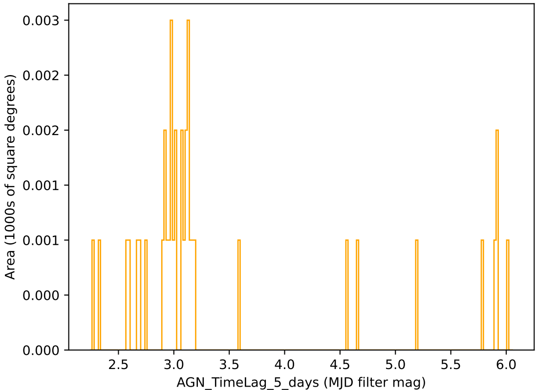
weather_cloudso20v3.4_10yrs r band: AGN_TimeLag_5_days
