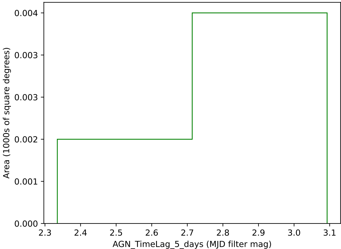
weather_cloudso20v3.4_10yrs g band: AGN_TimeLag_5_days
