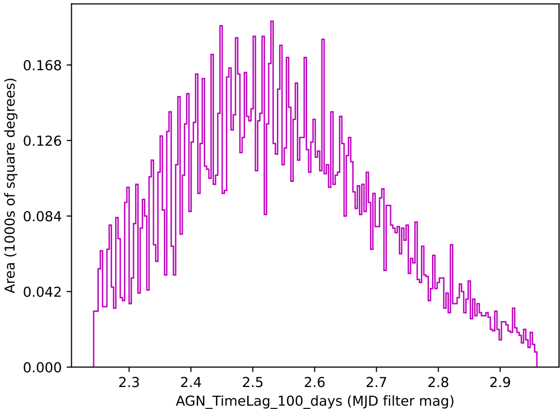
weather_cloudso20v3.4_10yrs z band: AGN_TimeLag_100_days
