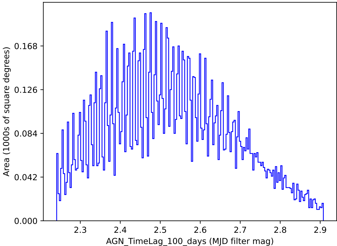
weather_cloudso20v3.4_10yrs y band: AGN_TimeLag_100_days
