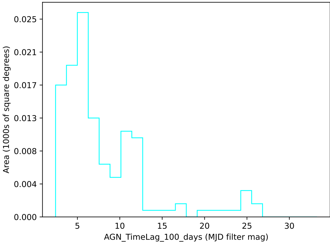
weather_cloudso20v3.4_10yrs u band: AGN_TimeLag_100_days
