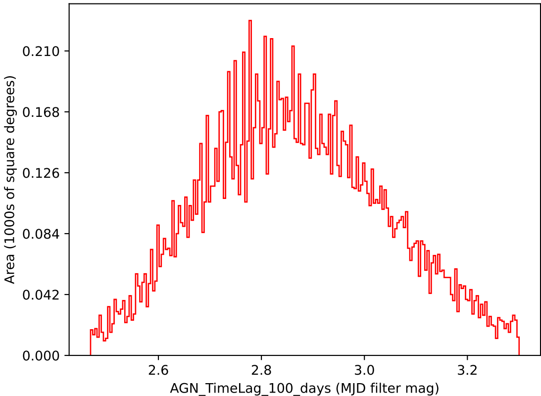
weather_cloudso20v3.4_10yrs i band: AGN_TimeLag_100_days
