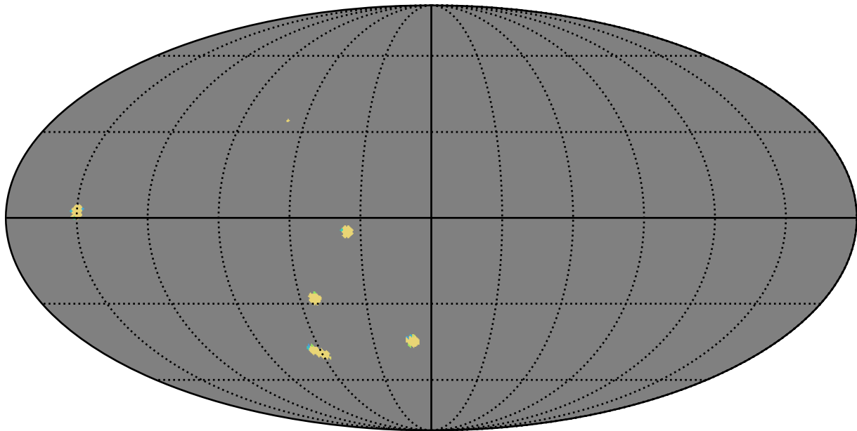
weather_cloudso20v3.4_10yrs g band: AGN_TimeLag_100_days
