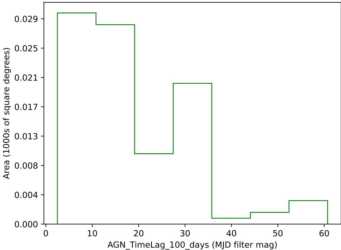
weather_cloudso20v3.4_10yrs g band: AGN_TimeLag_100_days
