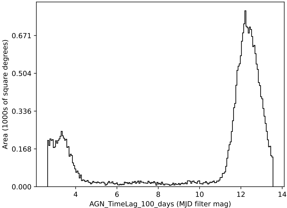
weather_cloudso20v3.4_10yrs all bands: AGN_TimeLag_100_days
