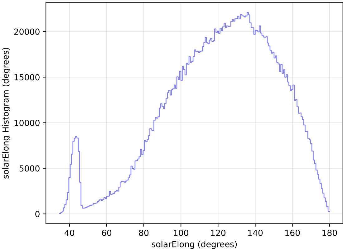
weather_cloudso20v3.4_10yrs WFD all bands: solarElong Histogram
