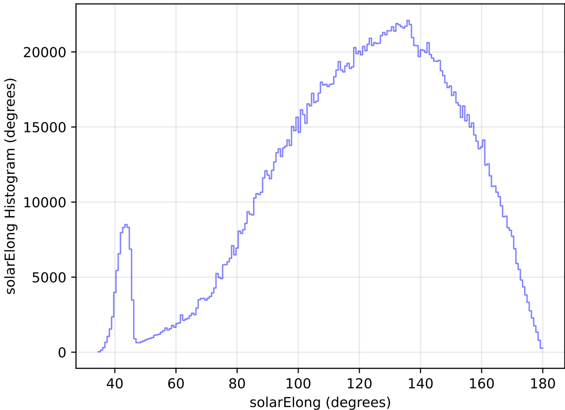
weather_cloudso20v3.4_10yrs All sky all bands: solarElong Histogram
