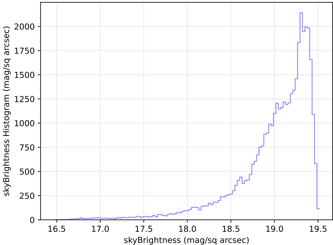
weather_cloudso20v3.4_10yrs Yr 1 z band: skyBrightness Histogram
