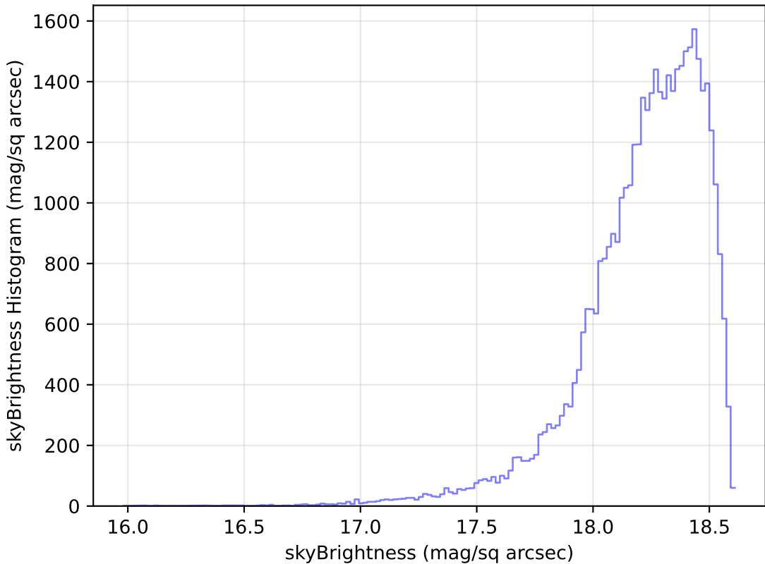
weather_cloudso20v3.4_10yrs Yr 1 y band: skyBrightness Histogram
