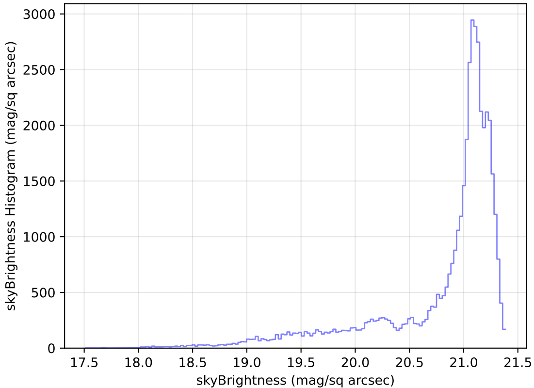
weather_cloudso20v3.4_10yrs Yr 1 r band: skyBrightness Histogram
