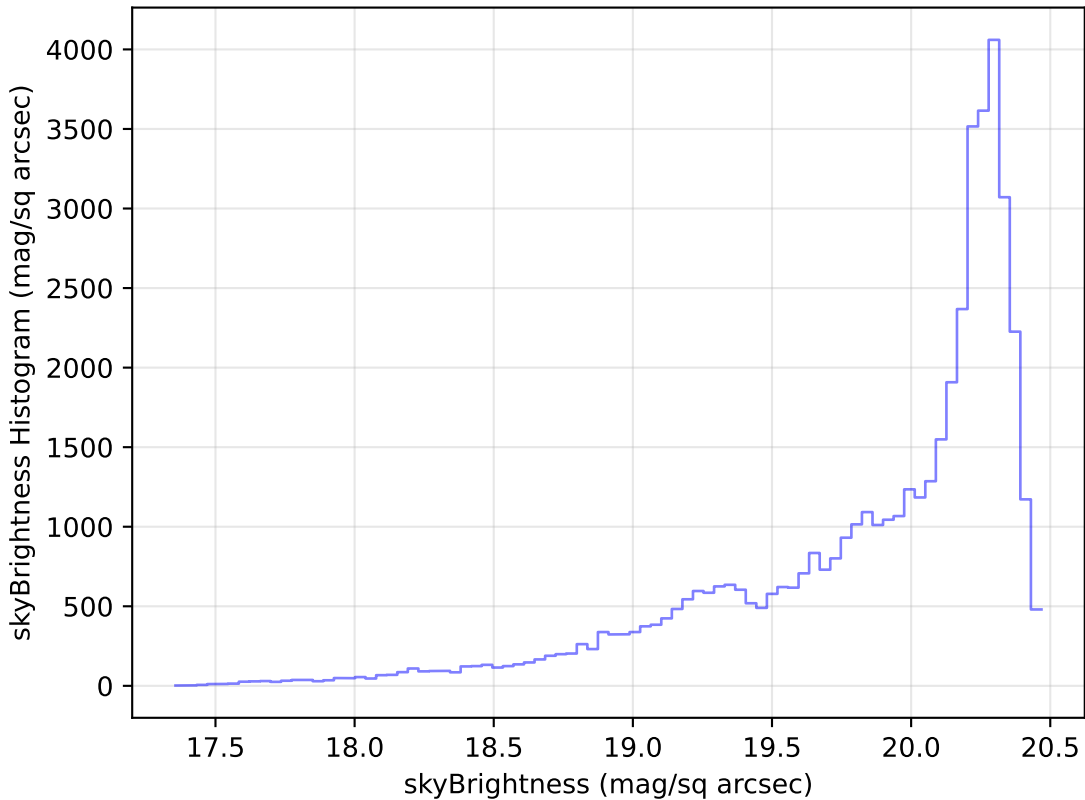
weather_cloudso20v3.4_10yrs Yr 1 i band: skyBrightness Histogram
