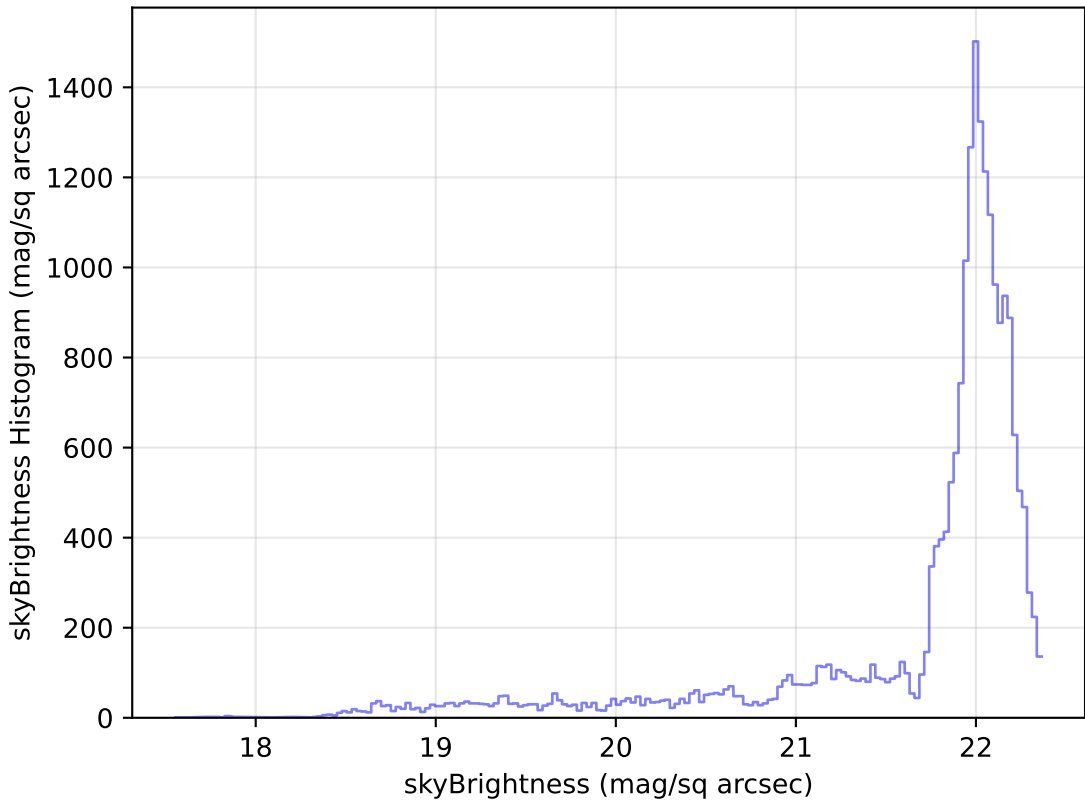
weather_cloudso20v3.4_10yrs Yr 1 g band: skyBrightness Histogram
