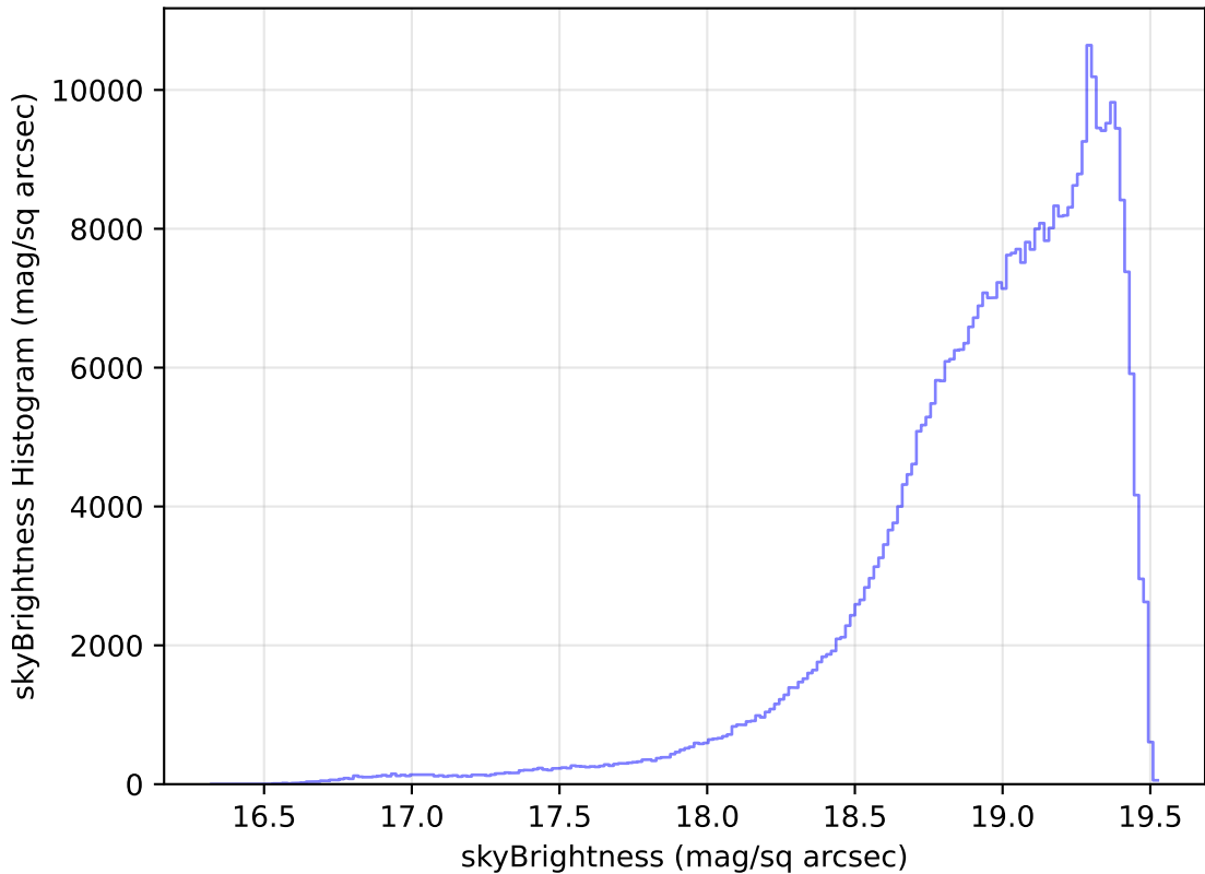
weather_cloudso20v3.4_10yrs WFD z band: skyBrightness Histogram
