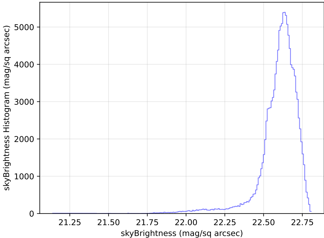
weather_cloudso20v3.4_10yrs WFD u band: skyBrightness Histogram
