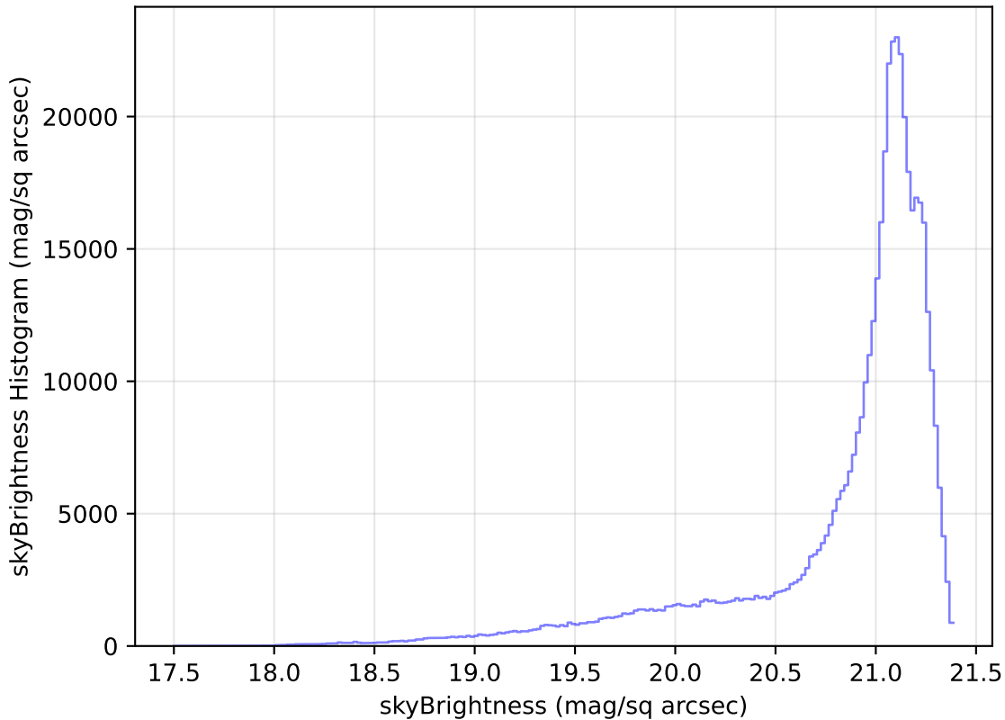
weather_cloudso20v3.4_10yrs WFD r band: skyBrightness Histogram
