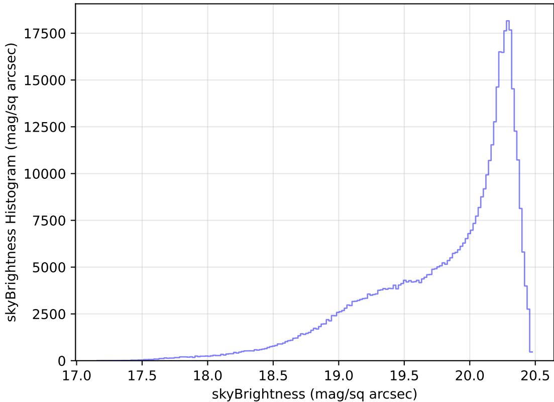
weather_cloudso20v3.4_10yrs WFD i band: skyBrightness Histogram
