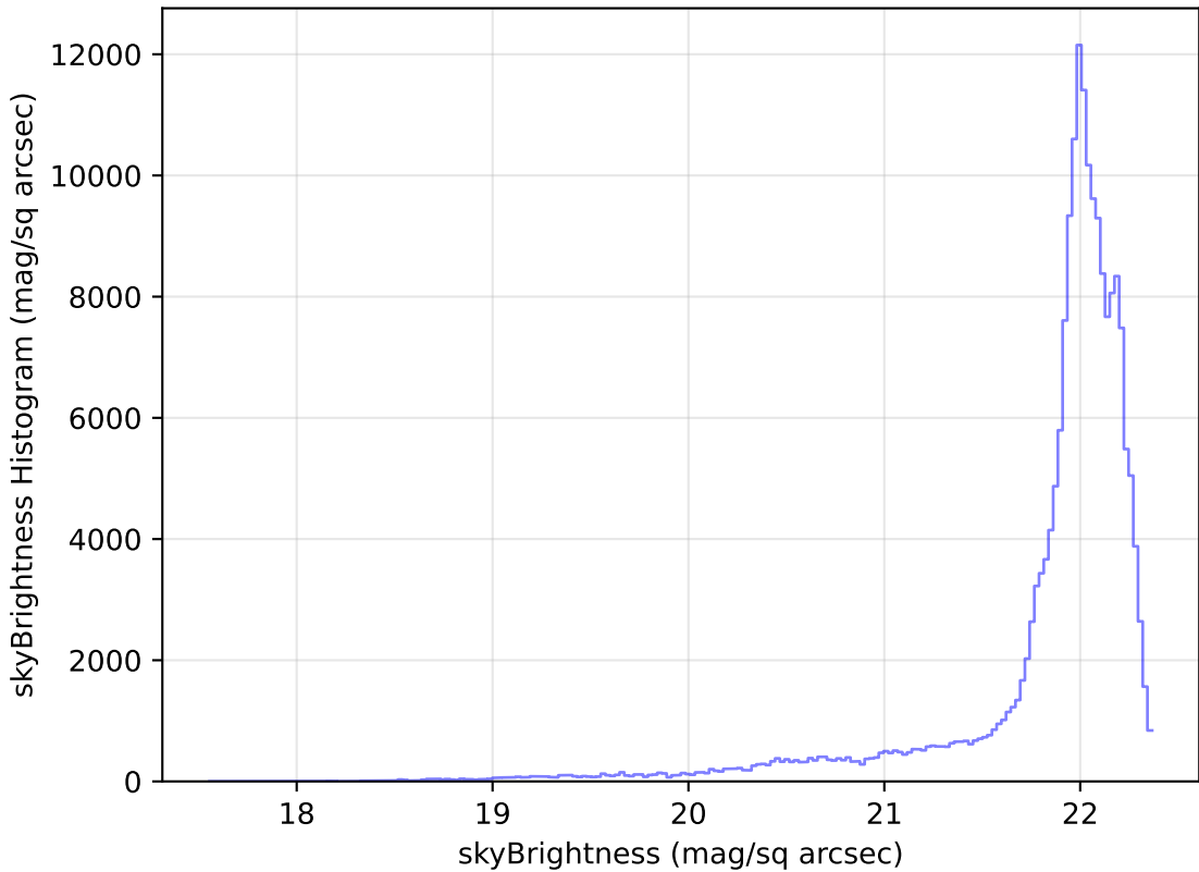
weather_cloudso20v3.4_10yrs WFD g band: skyBrightness Histogram
