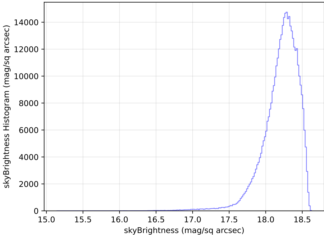
weather_cloudso20v3.4_10yrs All sky y band: skyBrightness Histogram
