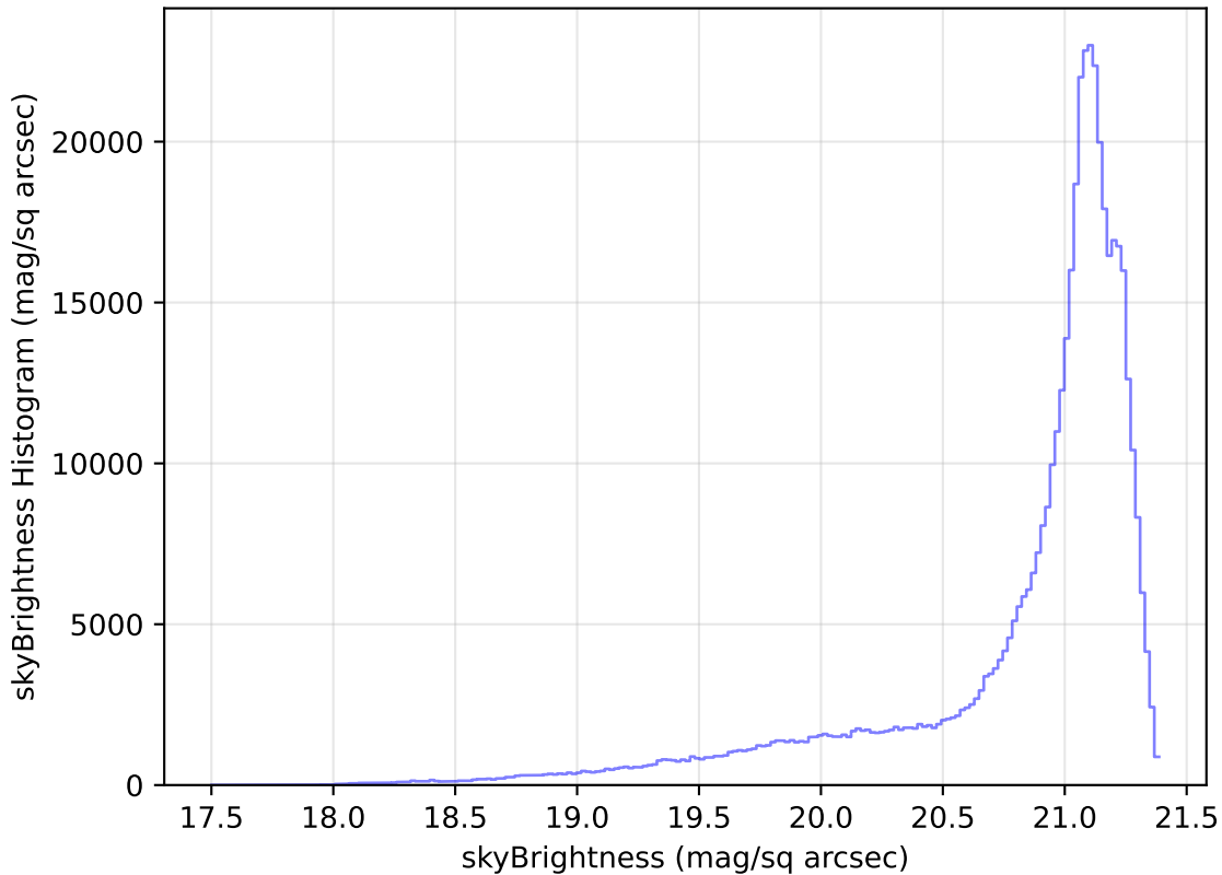
weather_cloudso20v3.4_10yrs All sky r band: skyBrightness Histogram
