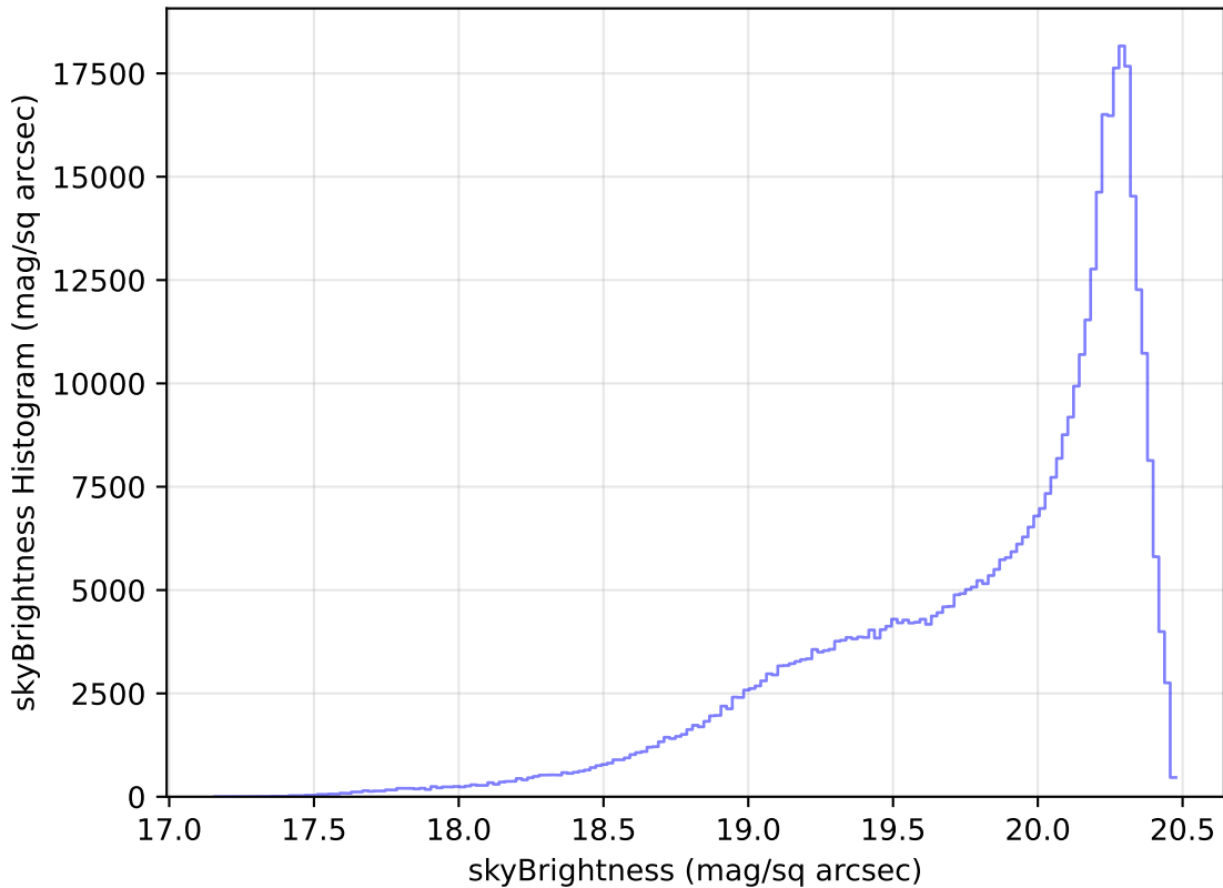
weather_cloudso20v3.4_10yrs All sky i band: skyBrightness Histogram
