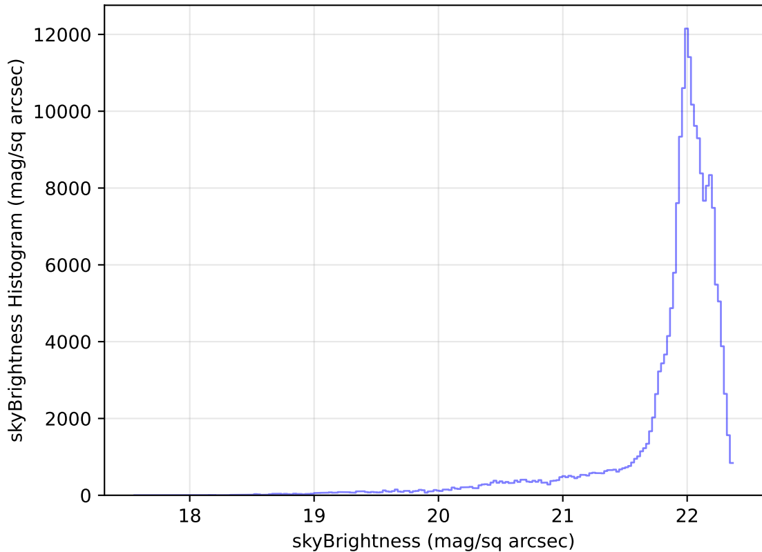
weather_cloudso20v3.4_10yrs All sky g band: skyBrightness Histogram
