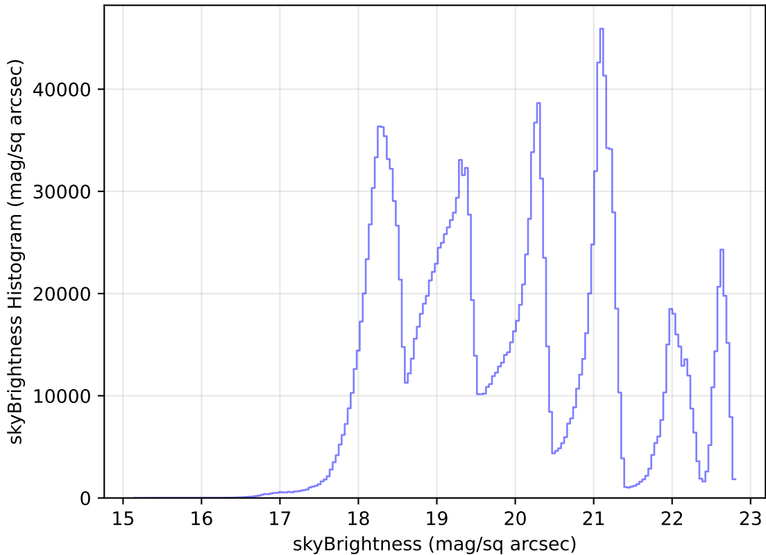
weather_cloudso20v3.4_10yrs All sky all bands: skyBrightness Histogram
