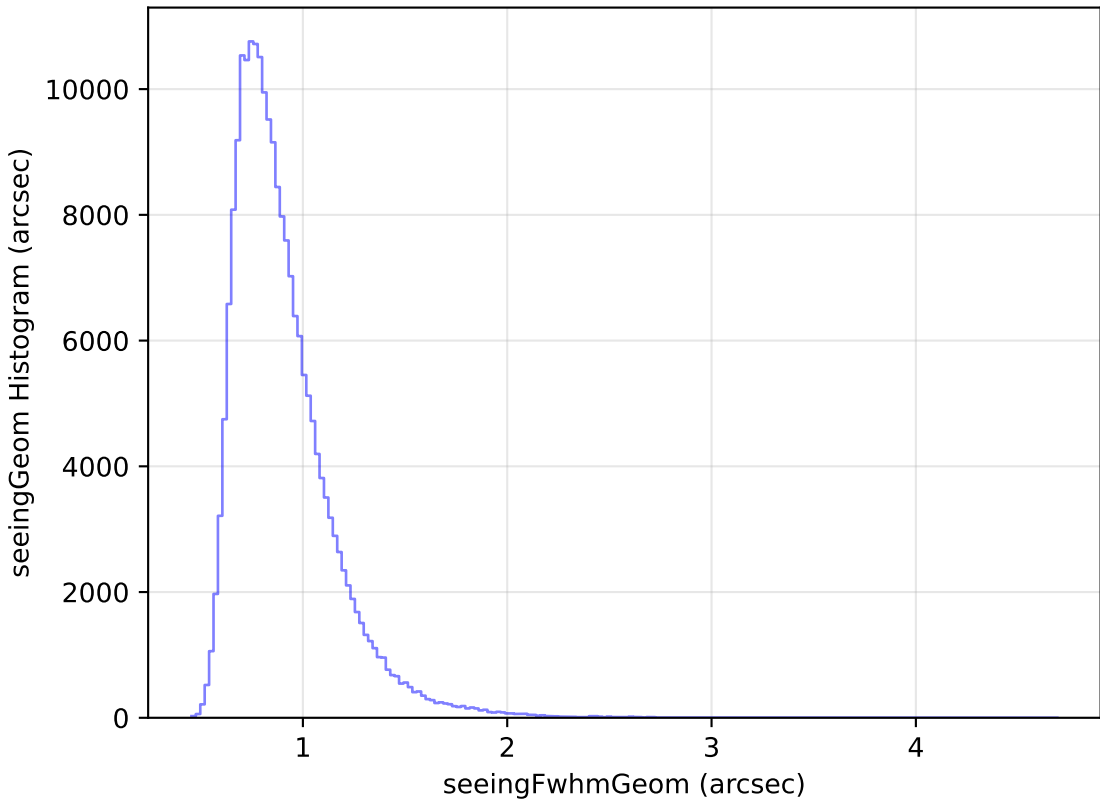
weather_cloudso20v3.4_10yrs Yr 1 all bands: seeingGeom Histogram
