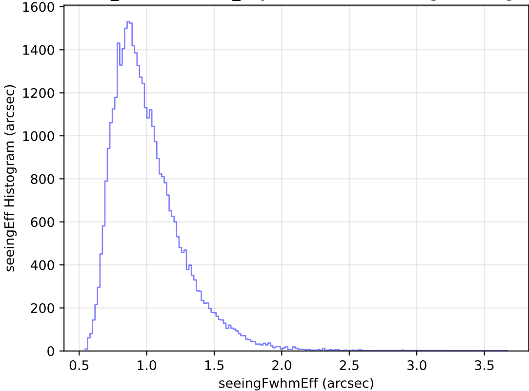
weather_cloudso20v3.4_10yrs Yr 1 z band: seeingEff Histogram
