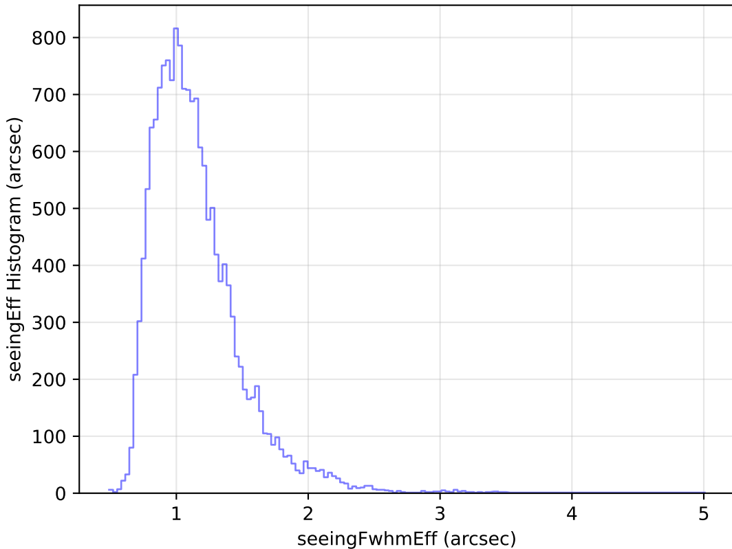
weather_cloudso20v3.4_10yrs Yr 1 u band: seeingEff Histogram
