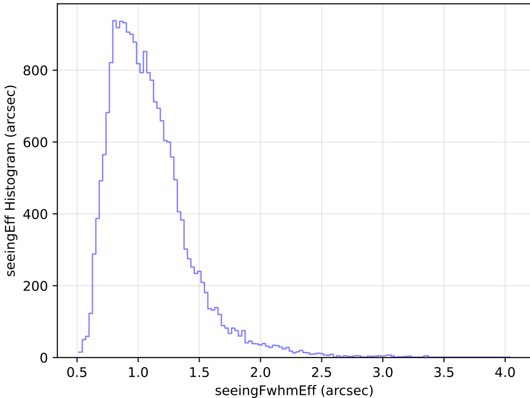
weather_cloudso20v3.4_10yrs Yr 1 g band: seeingEff Histogram
