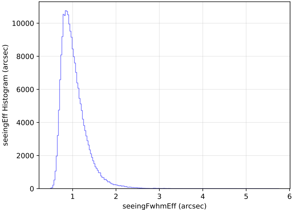
weather_cloudso20v3.4_10yrs Yr 1 all bands: seeingEff Histogram
