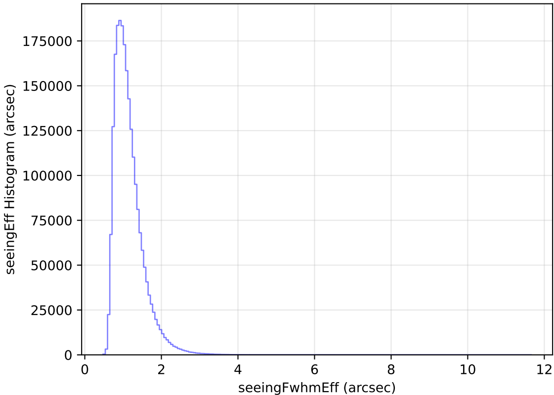
weather_cloudso20v3.4_10yrs WFD all bands: seeingEff Histogram
