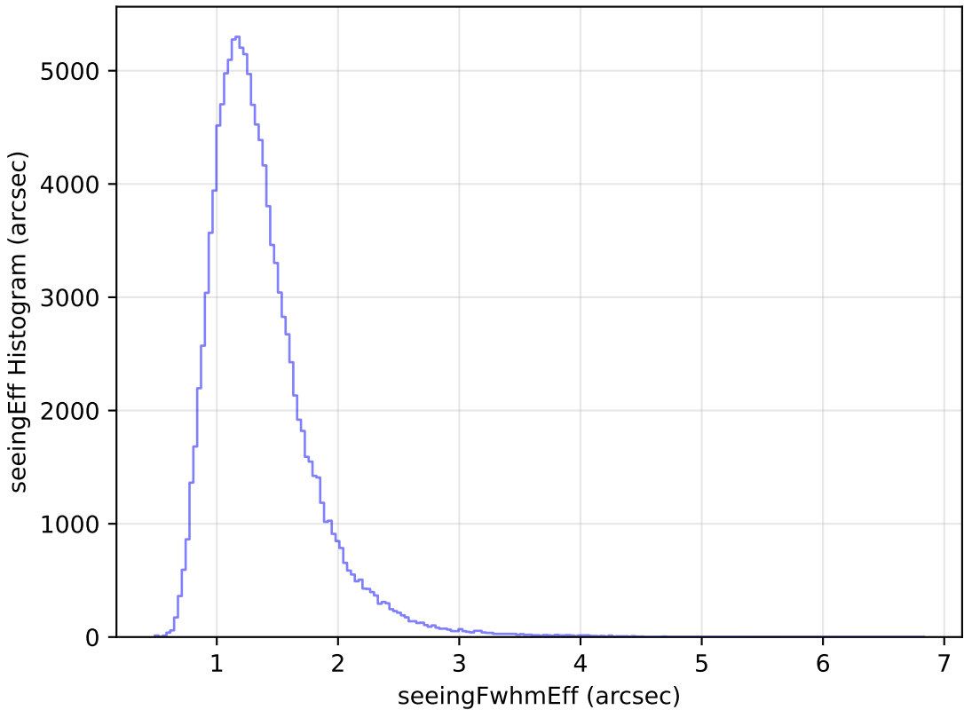
weather_cloudso20v3.4_10yrs All sky u band: seeingEff Histogram
