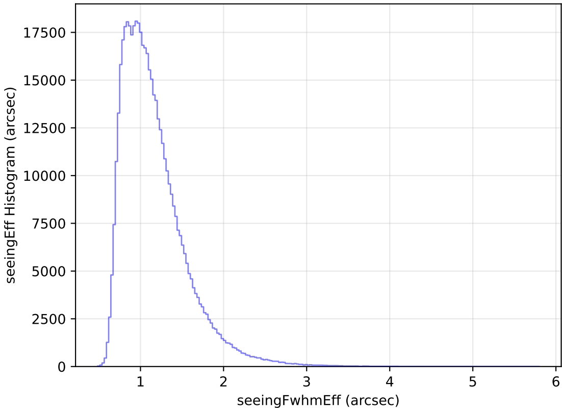
weather_cloudso20v3.4_10yrs All sky r band: seeingEff Histogram
