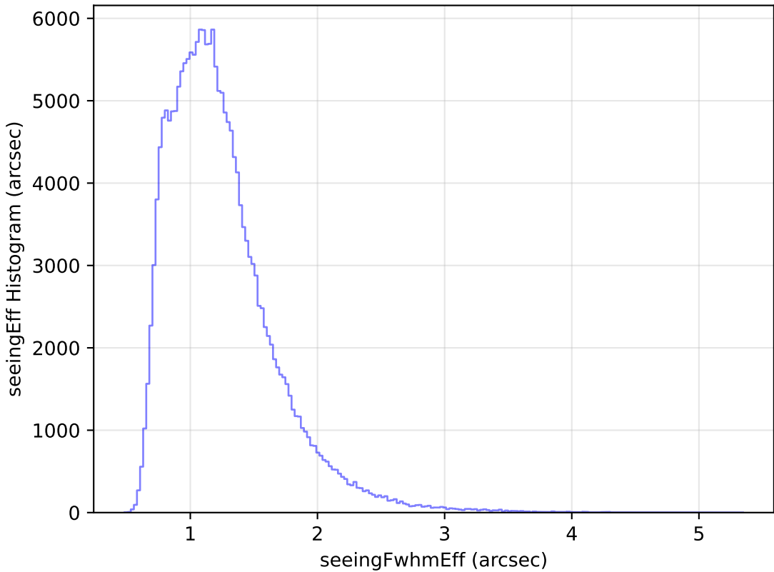
weather_cloudso20v3.4_10yrs All sky g band: seeingEff Histogram
