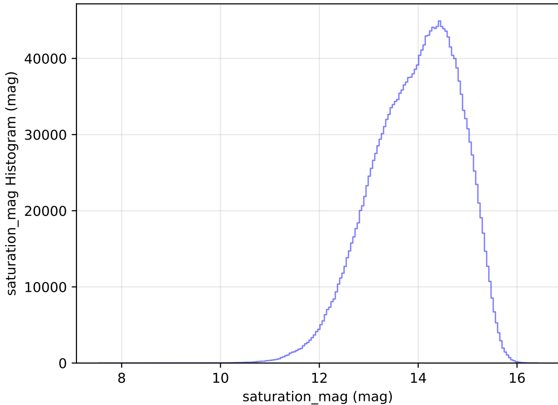
weather_cloudso20v3.4_10yrs WFD all bands: saturation_mag Histogram
