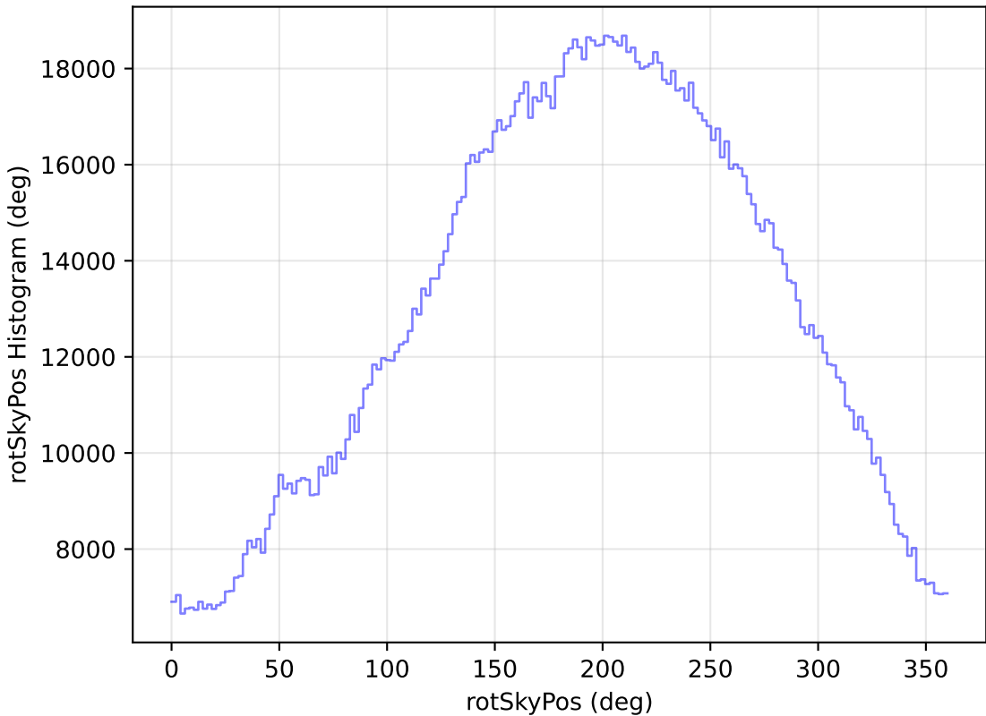
weather_cloudso20v3.4_10yrs WFD all bands: rotSkyPos Histogram
