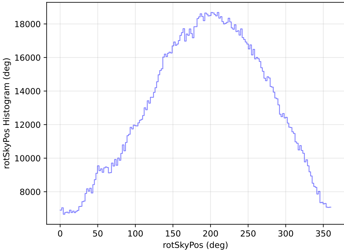
weather_cloudso20v3.4_10yrs All sky all bands: rotSkyPos Histogram
