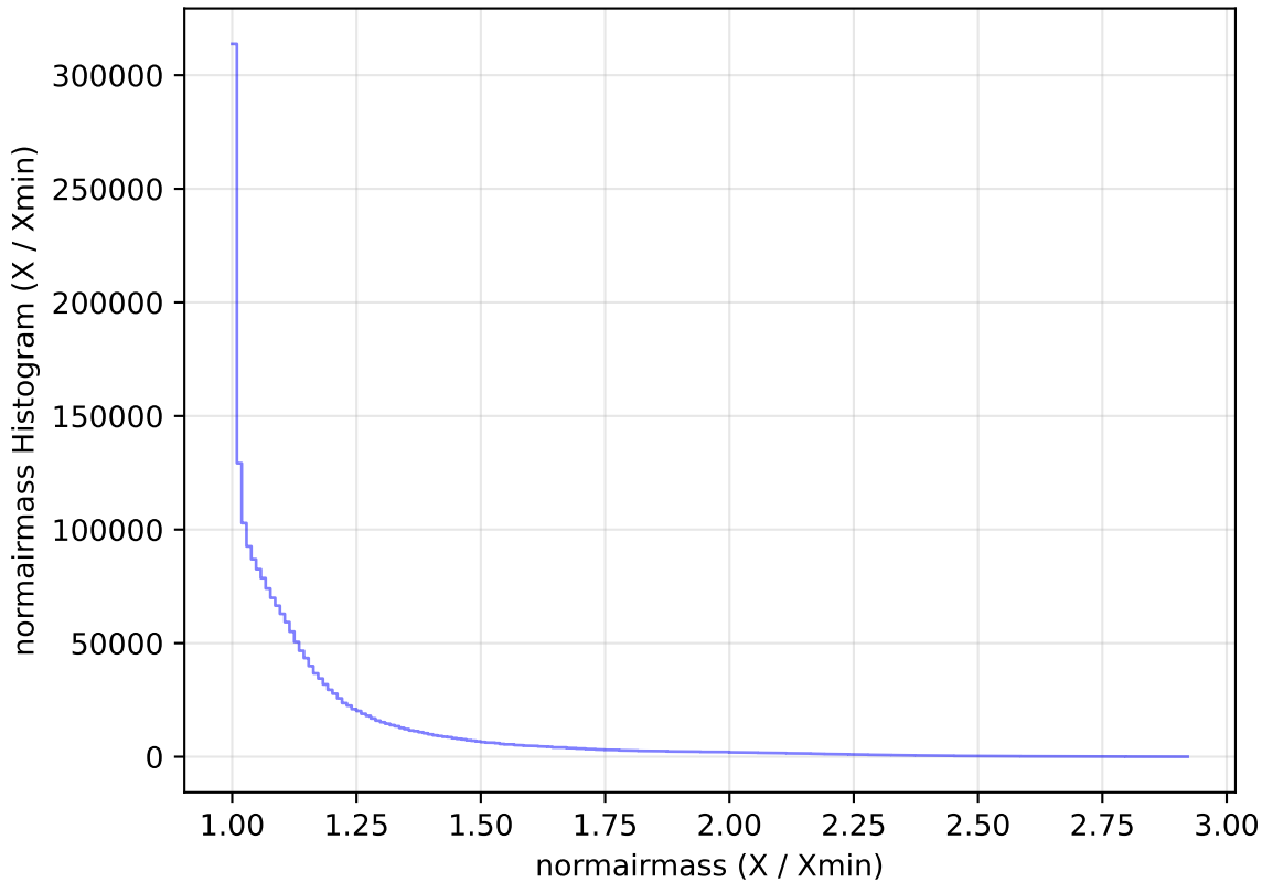
weather_cloudso20v3.4_10yrs WFD all bands: normairmass Histogram
