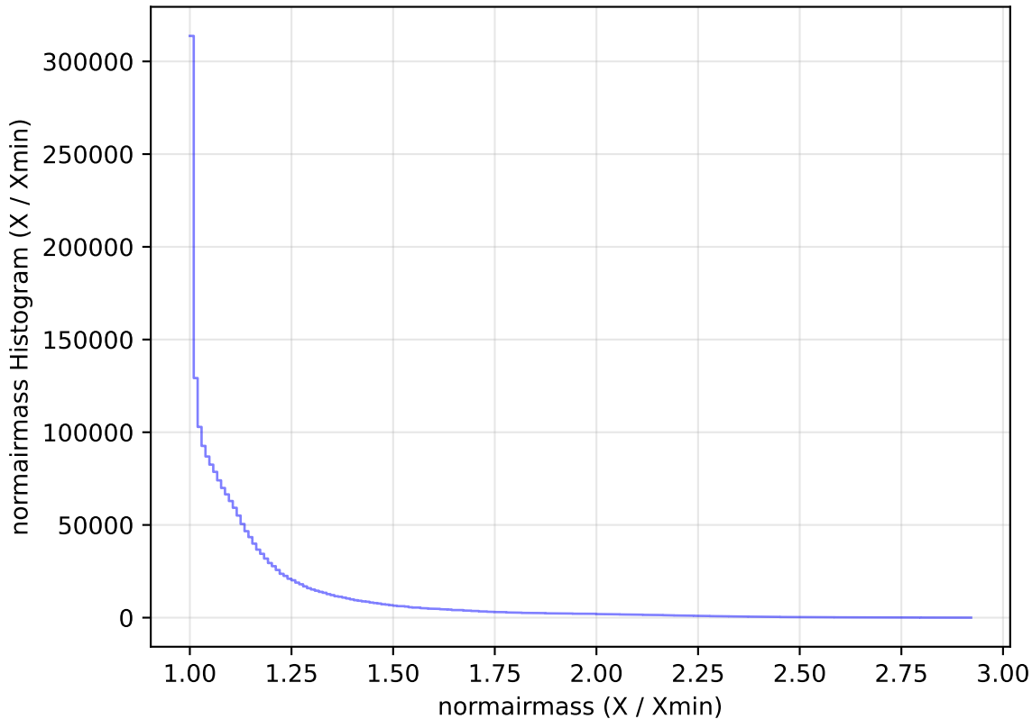
weather_cloudso20v3.4_10yrs All sky all bands: normairmass Histogram
