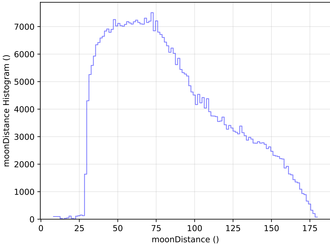
weather_cloudso20v3.4_10yrs WFD z band: moonDistance Histogram
