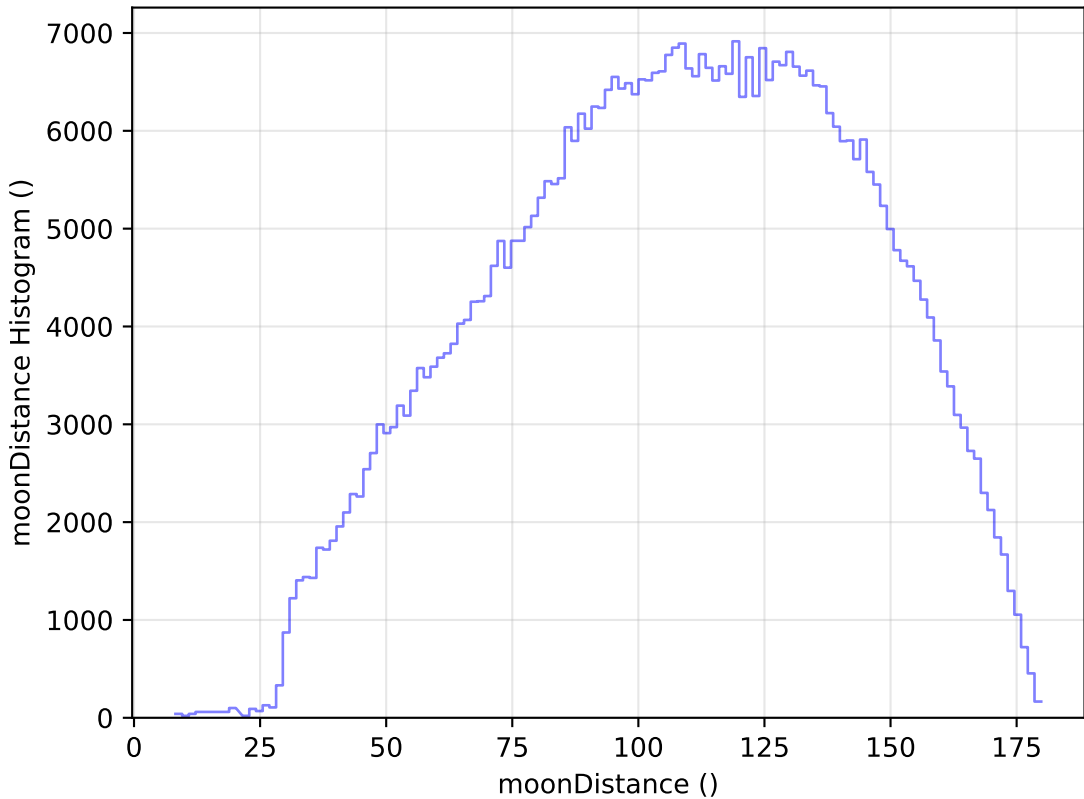
weather_cloudso20v3.4_10yrs WFD r band: moonDistance Histogram
