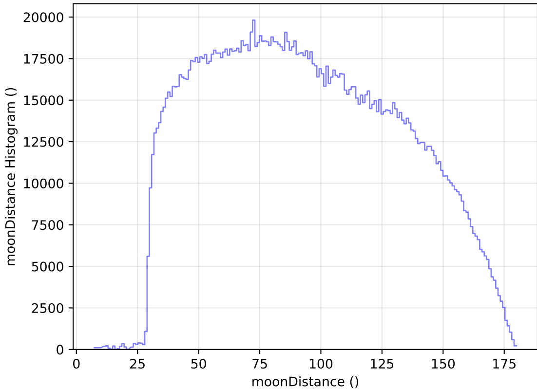
weather_cloudso20v3.4_10yrs WFD all bands: moonDistance Histogram
