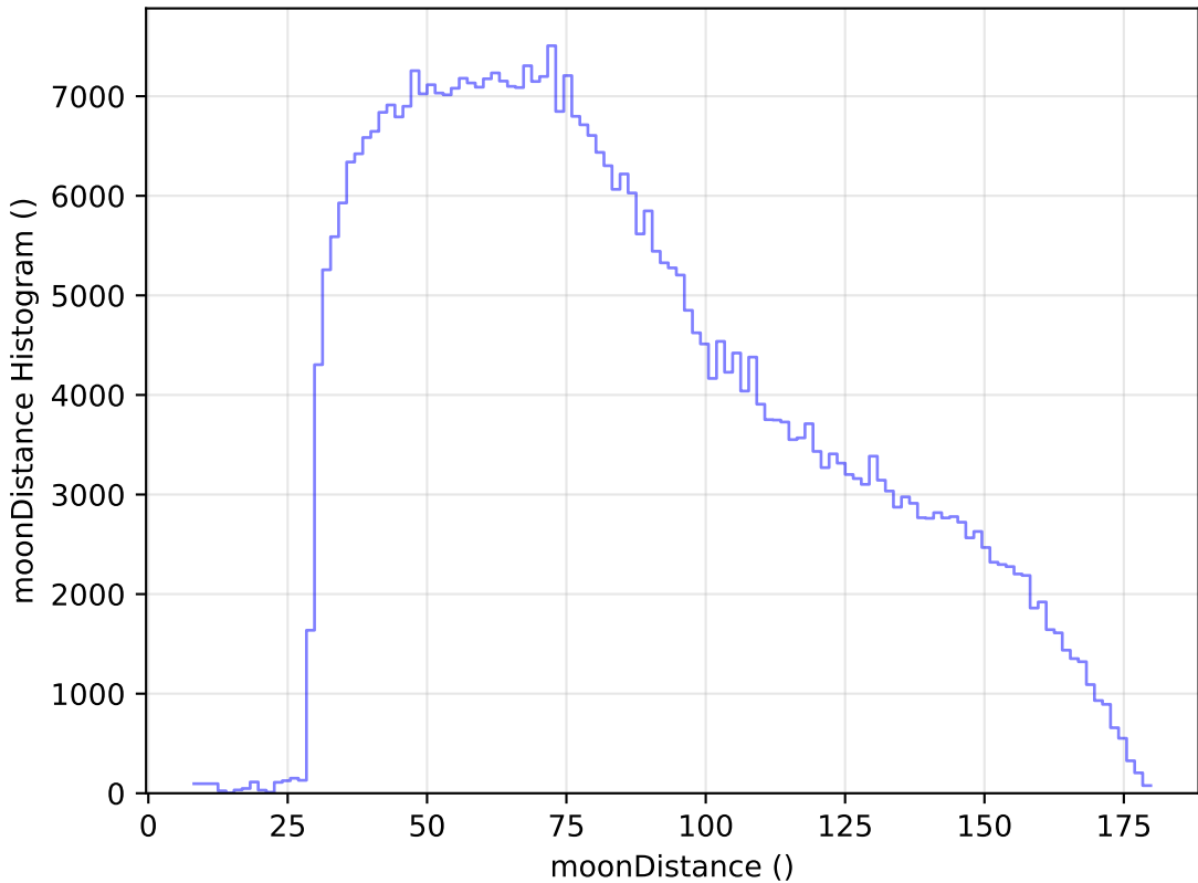
weather_cloudso20v3.4_10yrs All sky z band: moonDistance Histogram
