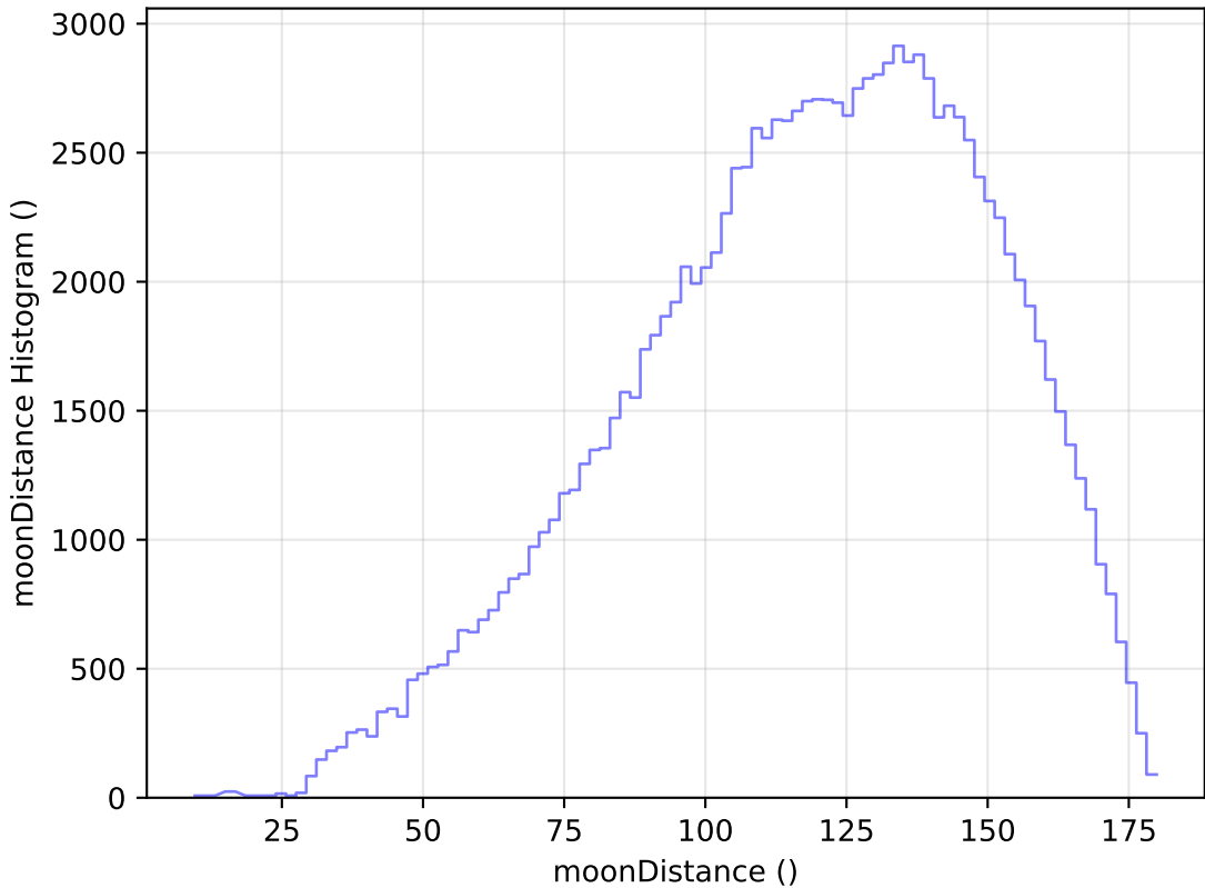
weather_cloudso20v3.4_10yrs All sky u band: moonDistance Histogram
