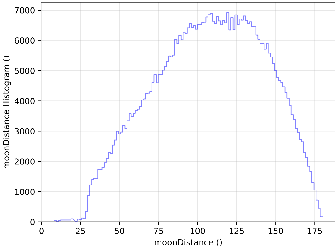
weather_cloudso20v3.4_10yrs All sky r band: moonDistance Histogram
