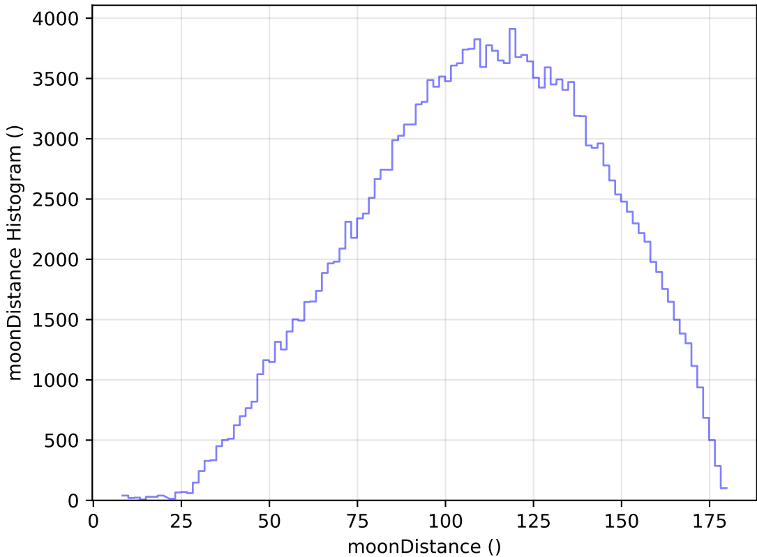
weather_cloudso20v3.4_10yrs All sky g band: moonDistance Histogram
