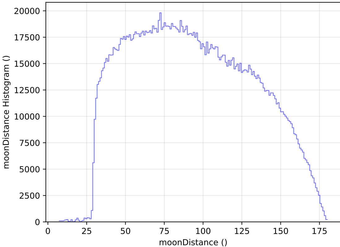
weather_cloudso20v3.4_10yrs All sky all bands: moonDistance Histogram
