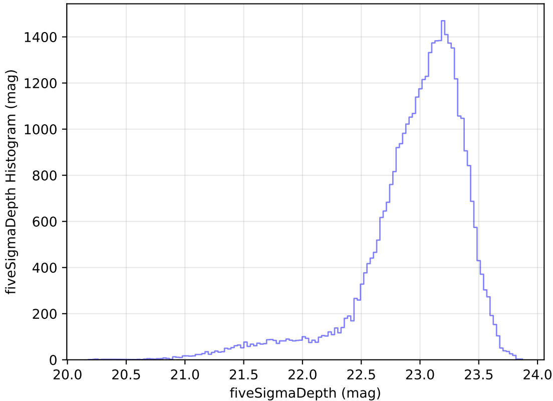
weather_cloudso20v3.4_10yrs Yr 1 z band: fiveSigmaDepth Histogram
