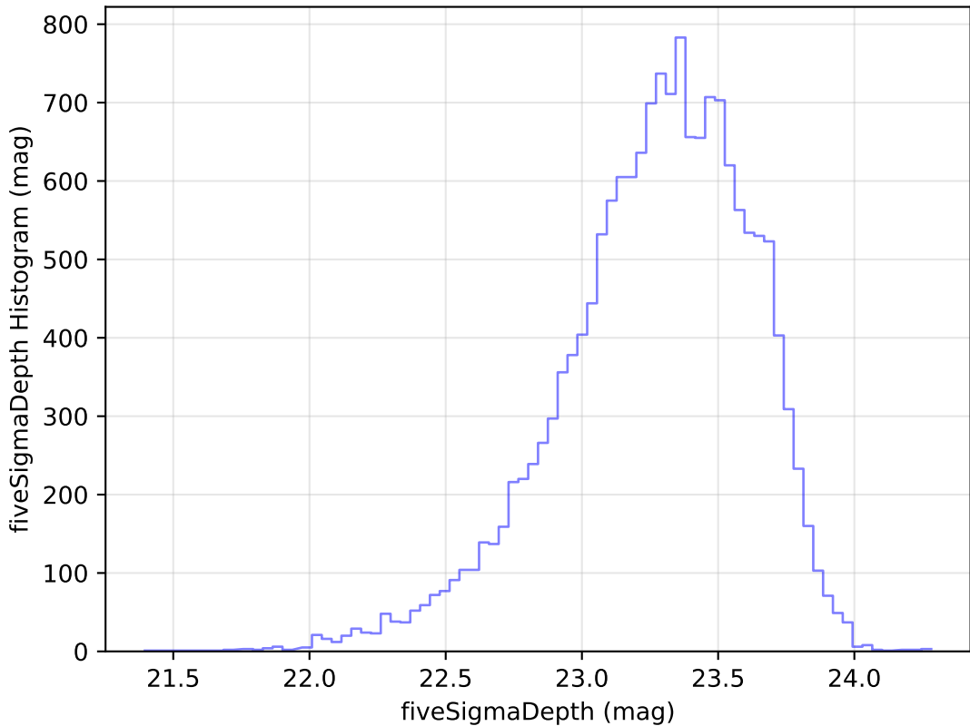
weather_cloudso20v3.4_10yrs Yr 1 u band: fiveSigmaDepth Histogram
